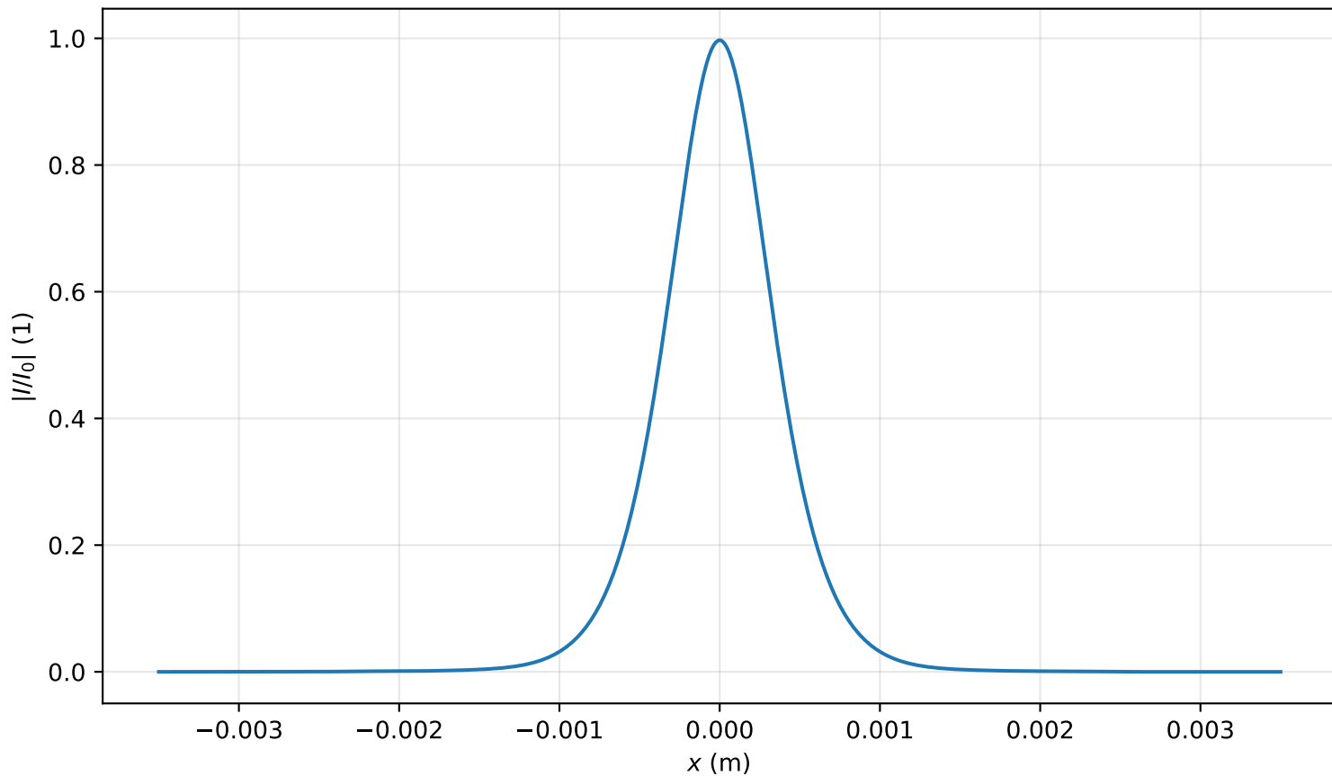
Intensity profile I(x, y = 0, z = 3.423m)/I_0 , P_{in}=0.8P_{cr} , artificial time
